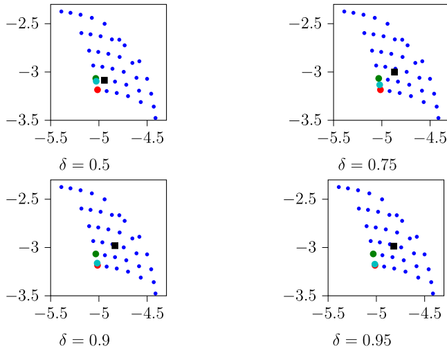
Fig. 5. Payoffs obtained for different values of the discount factor \delta in the distributed power control problem. The horizontal axis is V_1 , and the vertical axis V_2 . The small blue dots are the possible payoffs provided by all combinations of A_1 \times A_2 . The red point represents the NE payoff V_{n,k} : note that there are better payoffs for both players, i.e., points such that V_k > V_{n,k}, \forall k = 1, 2 . The green and cyan points have been obtained with the baseline, without deviation (green) and with the player 2 deviating in the second stage (cyan). The black square is the payoff obtained using LEWIS. Note how LEWIS is capable to obtain better payoffs than the baseline, and the improvement grows as \delta increases.
