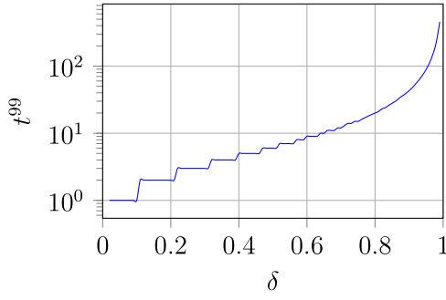
Fig. 1. Evolution of t^{99} as a function of \delta values using (4). The horizontal axis represents the \delta values, and in the vertical axis, we plot t^{99} , the number of stages needed to assign the 99% of the discounted payoff. Note that for low values of \delta most of the payoff is assigned in a few stages. Also, note that we may use (4) in order to obtain the discount factor in a game where t^M is a given parameter.
