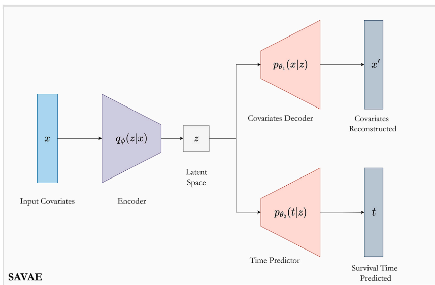
Fig. 1. Schematic representation of SAVAE. The encoder q_\phi(z|x) maps the input covariates x into a latent Gaussian space z . This latent space is used by a decoder p_{\theta_1}(x|z) , which reconstructs the covariates x , and a predictor p_{\theta_2}(t|z) , which estimates the survival time t .
